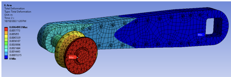
Fig. 10: Deformation chart of tensioning arm with ideal 4 kN loaded tension from the cable
