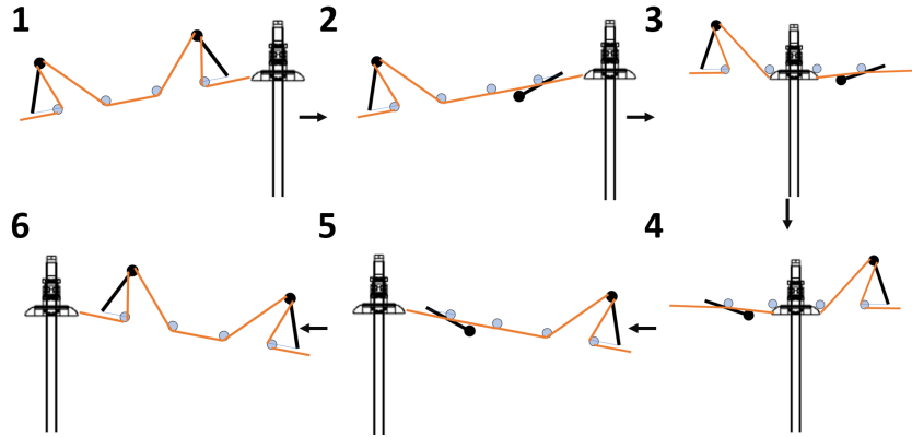
Fig. 12: Diagram breaking down the steps of a stake transition
