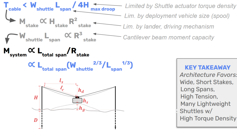
Fig. 3: Scaling laws that key system parameters follow
