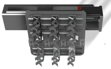
Fig. 8: Stake hand-off mechanism render
