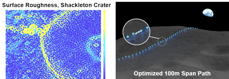
Fig. 18: Optimal path into Shackleton Crater with a 0.5 m ground clearance path and 100 m spans into Shackleton crater visualized (Saturn V for scale).
