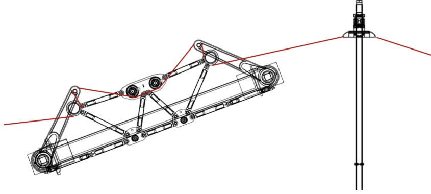
Fig. 11: Schematic of the shuttle approaching the cable for a stake transition
