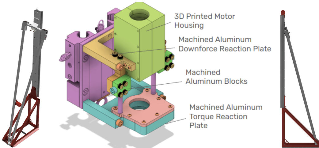
Fig. 7: Render of the entire elevator structure and the driver elevator interface
