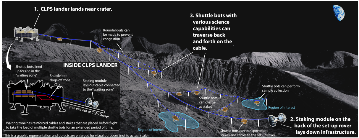
Fig. 6: Full pathfinder mission concept of operations
