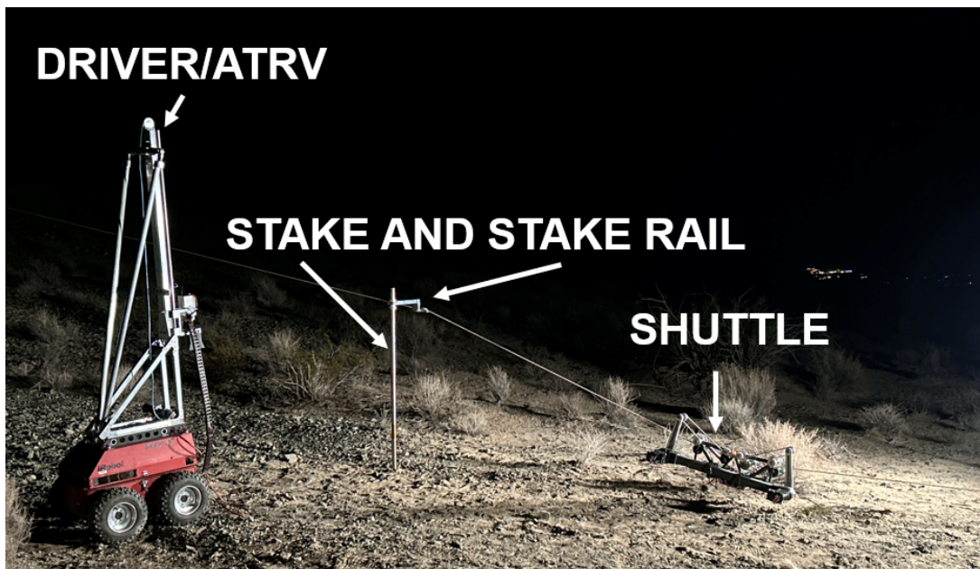
Fig. 1: Major system components at Lucerne Valley
