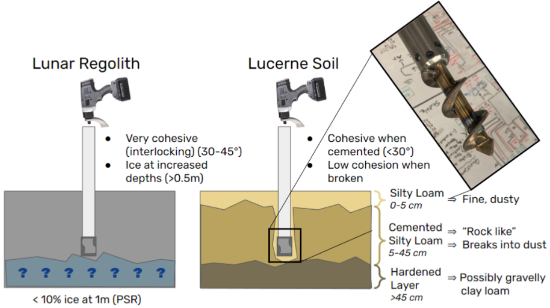
Fig. 14: Left: Stake in Lunar regolith. Right: Stake in Lucerne test site dirt
